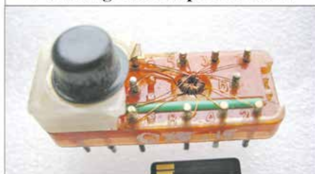
1 bit Magnetkernspeicher 1975
